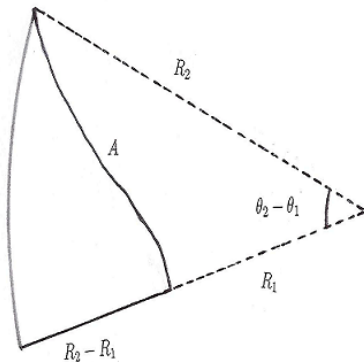
FIGURE 1. A curve A with finite length.
