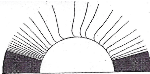
FIGURE 2. Trinomial curves L(p, k, r, n) .
